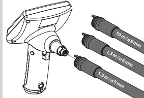
VideoFlex G2: MultiConnect system
